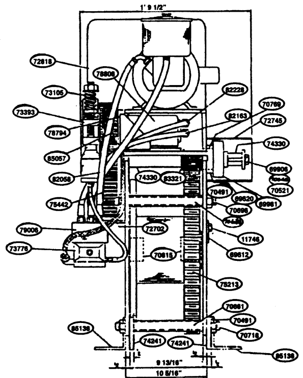
FRONT ELEVATION
